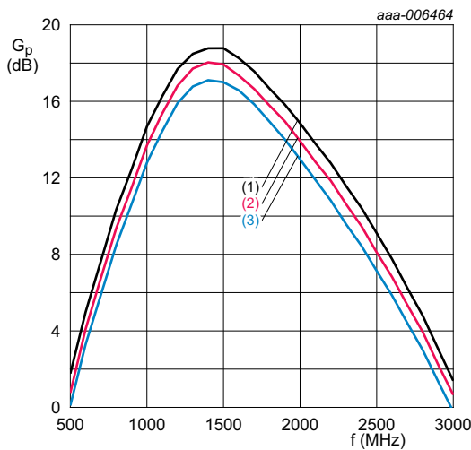
P_i = -45 dBm; V_{CC} = 1.8 V. (1) T_{amb} = -40^\circ\text{C} (2) T_{amb} = +25^\circ\text{C} (3) T_{amb} = +85^\circ\text{C}
