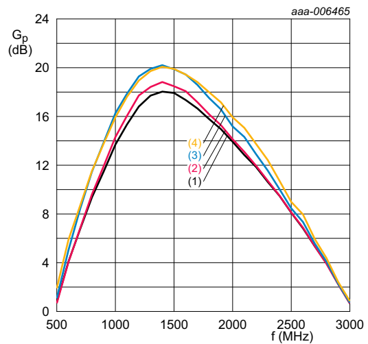
T_{amb} = 25^\circ\text{C} ; V_{CC} = 1.8 V. (1) P_i = -45 dBm (2) P_i = -30 dBm (3) P_i = -20 dBm (4) P_i = -15 dBm
