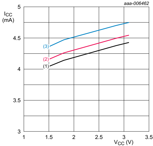
P_i = -45 dBm. (1) T_{amb} = -40^\circ\text{C} (2) T_{amb} = +25^\circ\text{C} (3) T_{amb} = +85^\circ\text{C}
